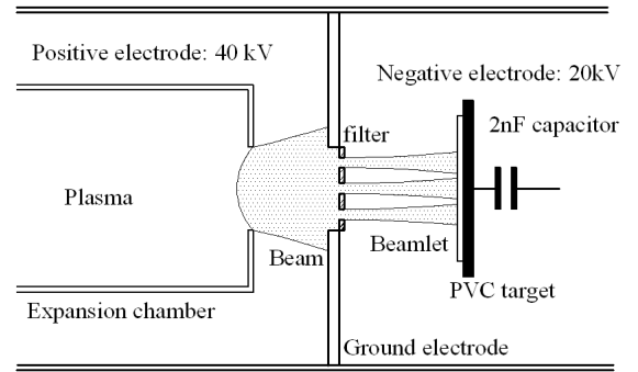
Fig. 5: Sketch of the pepper pot system .
